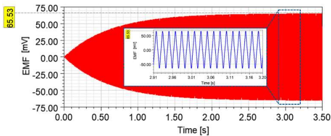
Fig. 6. Voltage output from the ECE model in an open circuit condition. The voltages between 2.91 s and 3.2 s are shown in the inner plot.
