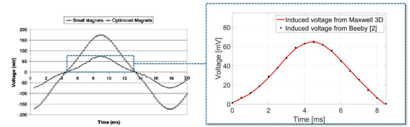
Fig. 4. Simulated output voltages from Beeby [2] (left) and Maxwell 3D transient analysis (right). The matching of the results as shown in this figure verifies the accuracy of our model built in Maxwell 3D.
