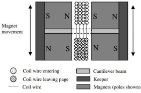
Fig. 2. Cross section through the four-magnet arrangement [2]. A concentrated flux gradient through the stationary coil is produced with this arrangement as the magnets vibrate.
