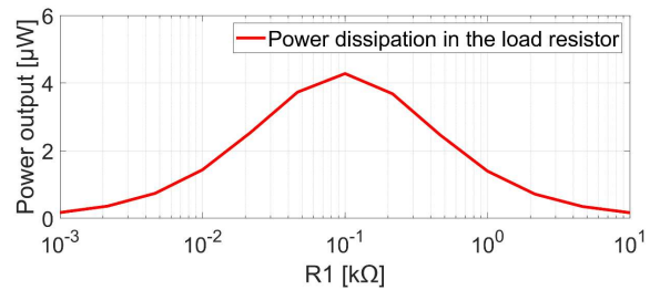
Fig. 7. Power dissipation in the load resistor with different values of load resistance. The maximum power is delivered when the load resistance equals the internal resistance of the coil at 100 \Omega .
